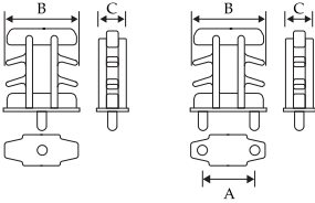
Solid Prong
